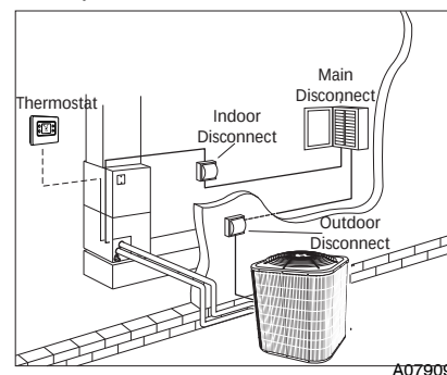
Fig. 1 - Electrical Disconnects
